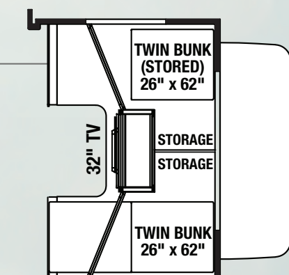
OPT. CABOVER TWIN BEDS W/ 32" TV 2251, 2291, 2301, 2501, 2651, 2701, 2861, 3011, 3051, 3171
