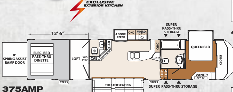
375AMP
