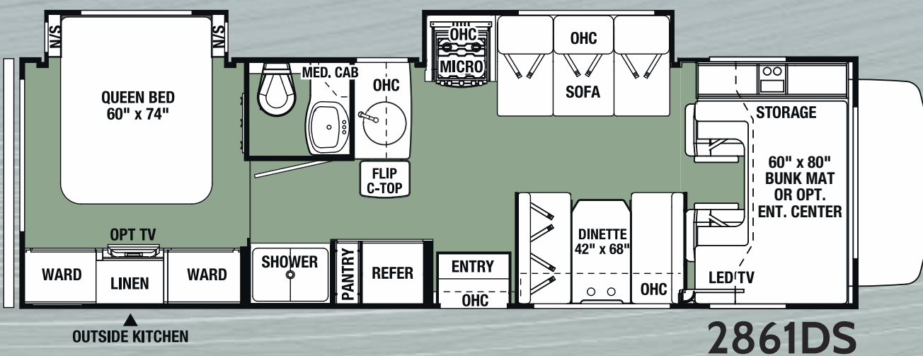
2861DS
