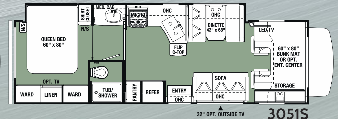
3051S
