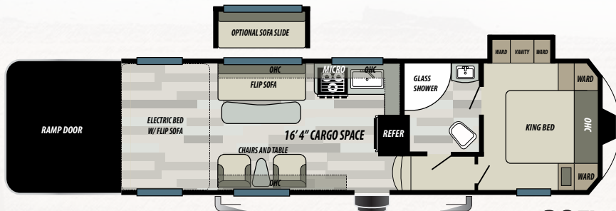
28FWGDX DRY WEIGHT 9,640 LBS
