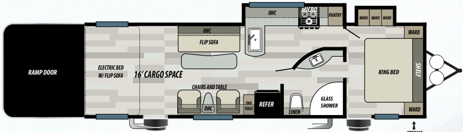
30KSGDX DRY WEIGHT 6,399 LBS
