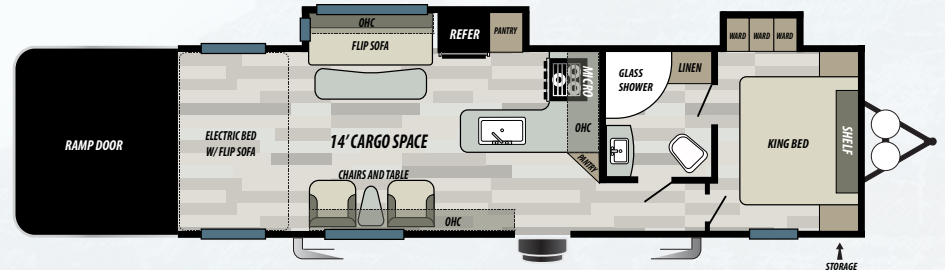
30KSGDX DRY WEIGHT 10,322 LBS
