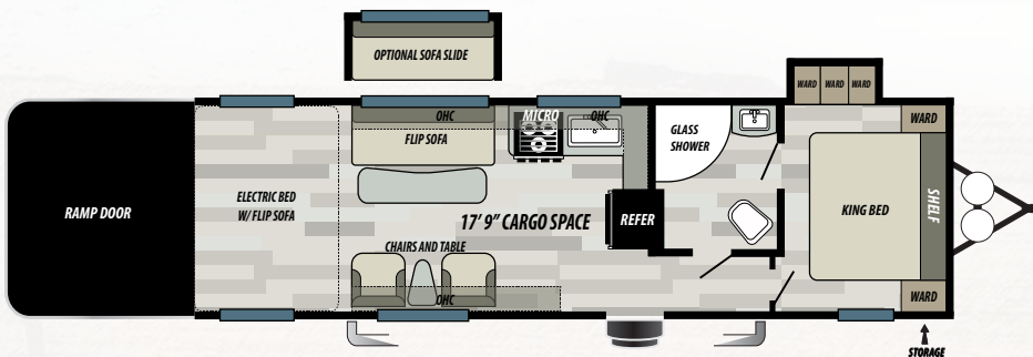
29RQDX DRY WEIGHT 9,108 LBS
