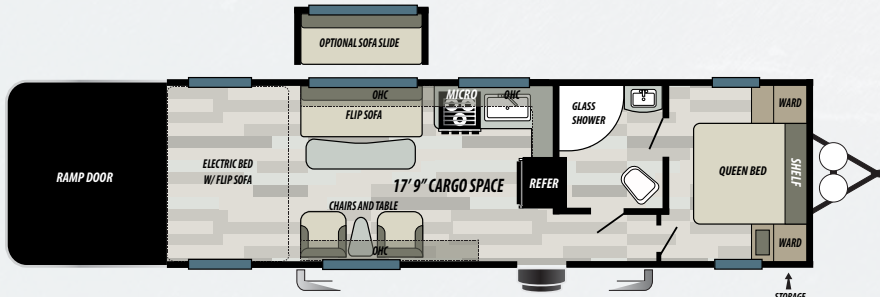
28RQDX DRY WEIGHT 8,212 LBS
