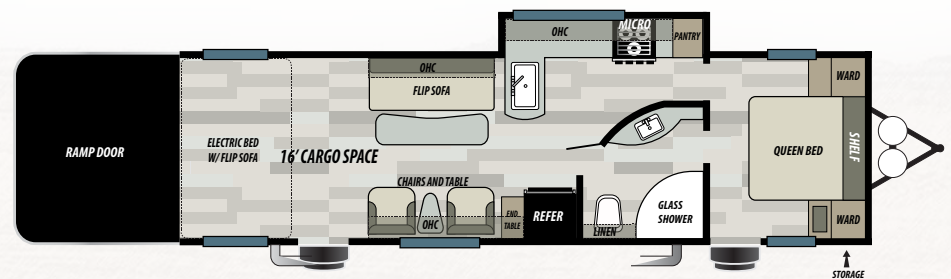
29KSGDX DRY WEIGHT 9,108 LBS
