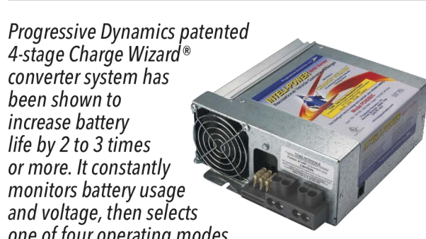
Progressive Dynamics patented 4-stage Charge Wizard® converter system has been shown to increase battery life by 2 to 3 times or more. It constantly monitors battery usage and voltage, then selects one of four operating modes to properly charge and maintain the battery. Boost, Normal, Storage and Equalization
